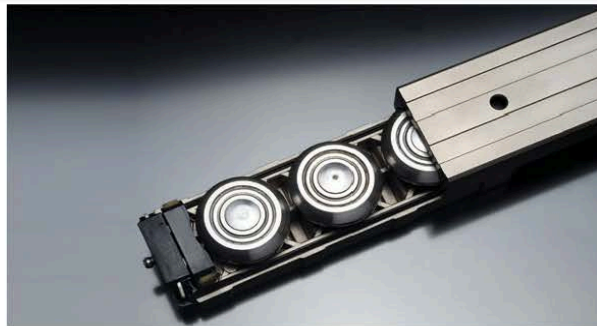
Rollon's Compact Rail system is inherently tolerant of misalignment, thanks to a rail geometry that can absorb alignment errors in one or two axes.
