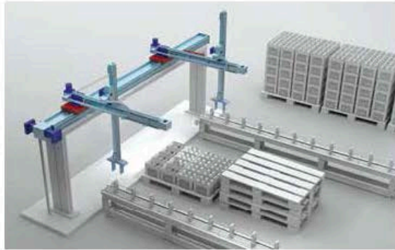
In certain end-of-line packaging scenarios, it makes sense to build a three-axis gantry system out of heavy-duty rigid actuators to handle heavy loads rather than using a SCARA robot with a more limited payload capacity.
